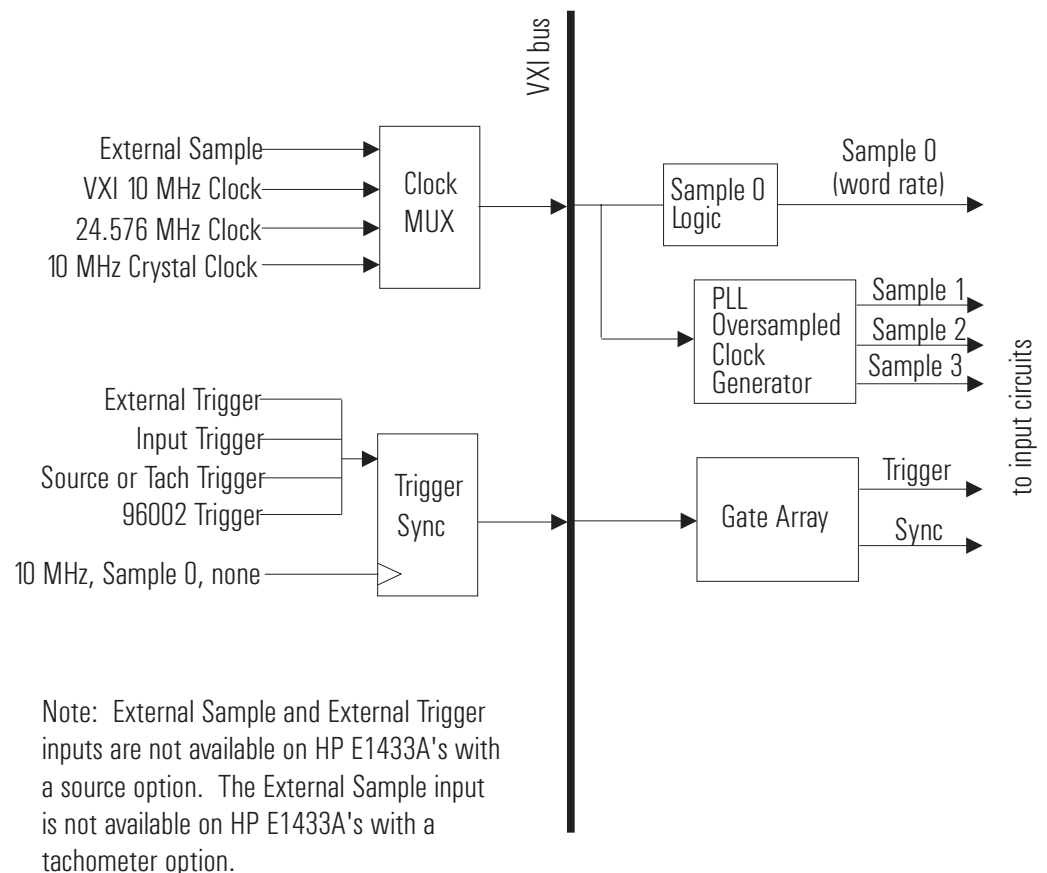
Figure 5-10: Clock/sync diagram
